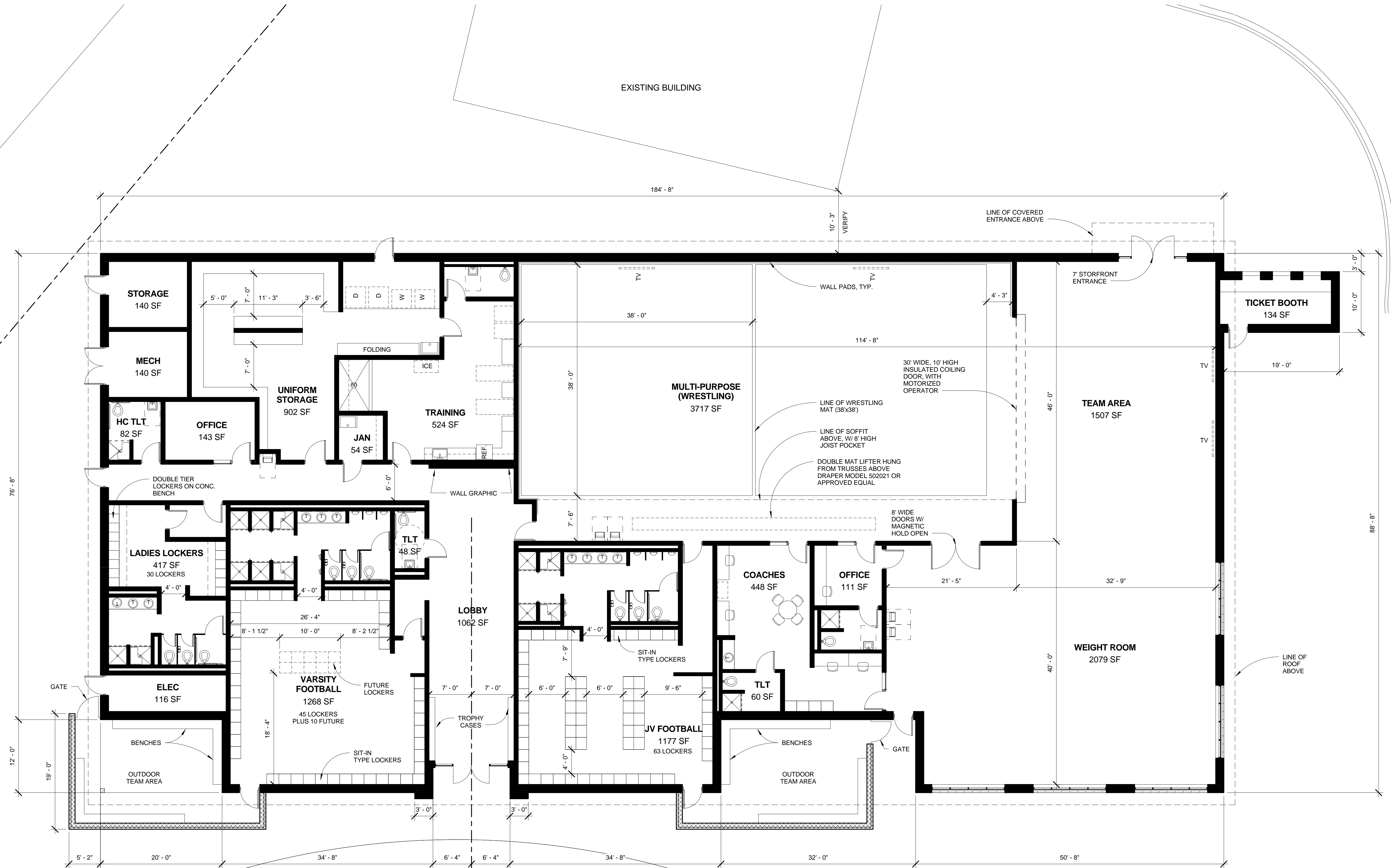
1 01 FIRST FLOOR PLAN -Scheme 4 1/8" = 1'-0" August 16, 2016
